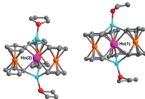
Fig. 2 Molecular structure of the two crystallographically unique [\text{HoFc}_3(\text{THF})_2\text{Li}_2]^- complexes of 2 . Hydrogen atoms and [\text{Li}(\text{THF})_4]^+ counter cations removed for clarity. Pink = Ho, orange = Fe, blue = Li, red = O, grey = C.
